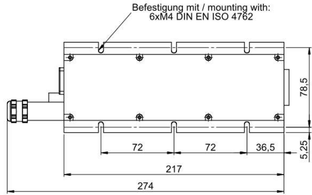
OEM-Controller
