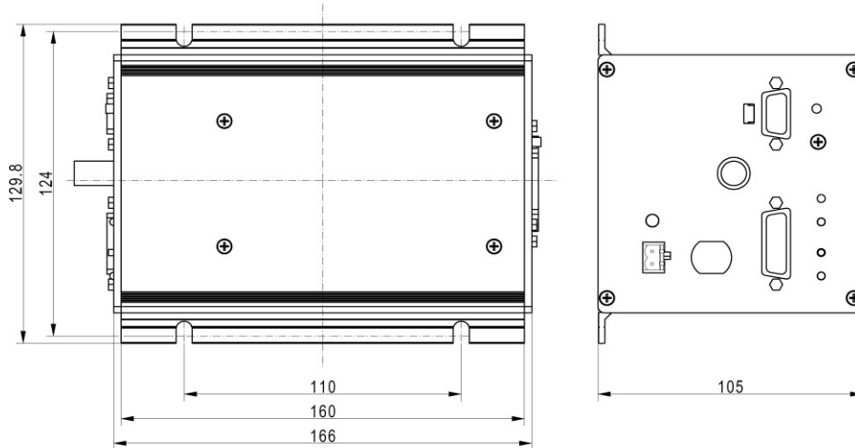
OEM-Controller
